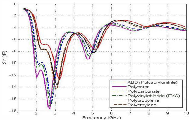
Figure 4. The Reflection Coefficients of Varieties Plastic Cover
