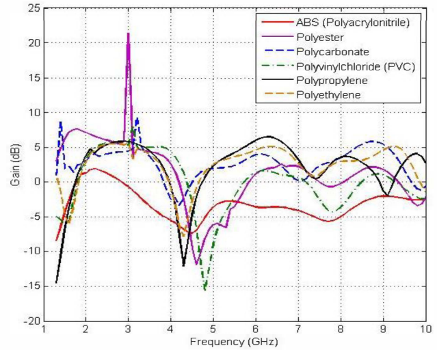
Figure 5. Antenna Gain Comparison for Various Plastic Cover
